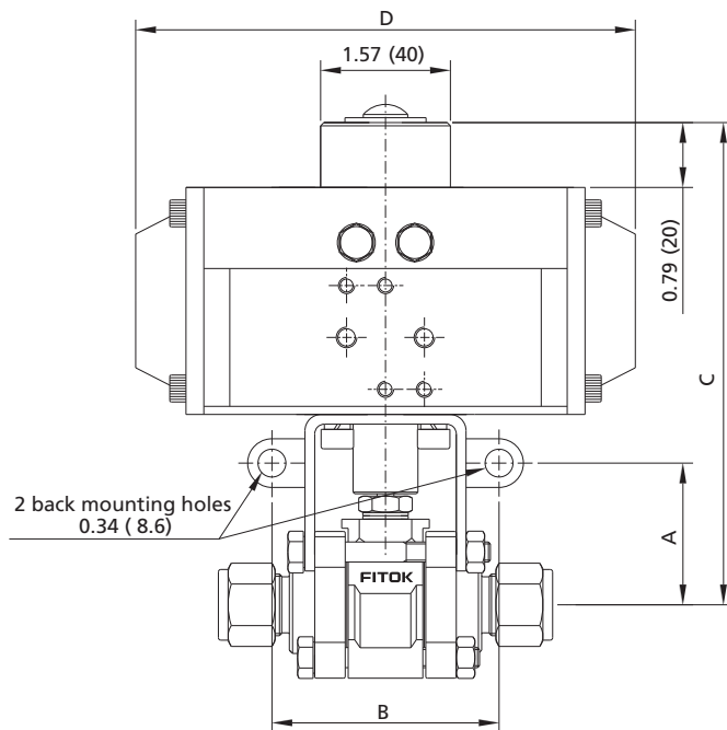
BH series ball valves
