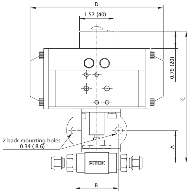
BF, BFH, BO, BP, BV series ball valves
