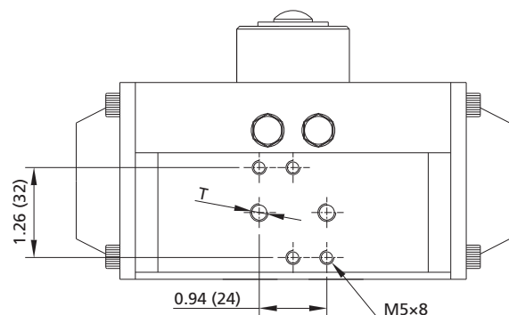
VDI/VDE 3845 (NAMUR) (View from Front)
