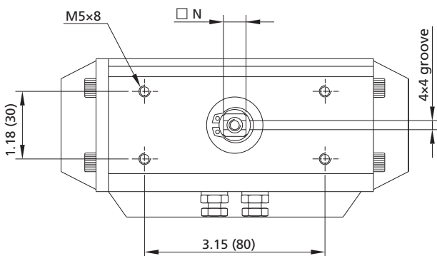
VDI/VDE 3845 (NAMUR) (View from Top)
