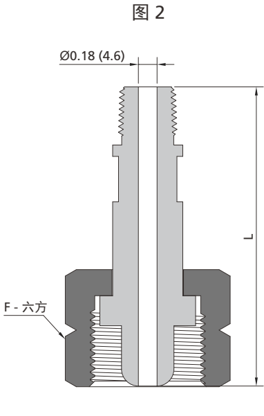
NPT 阳螺纹
